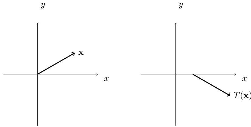
Figure 12.12: Glide reflections
