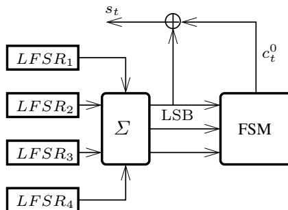
Fig. 1. The core of Bluetooth keystream generator E0
